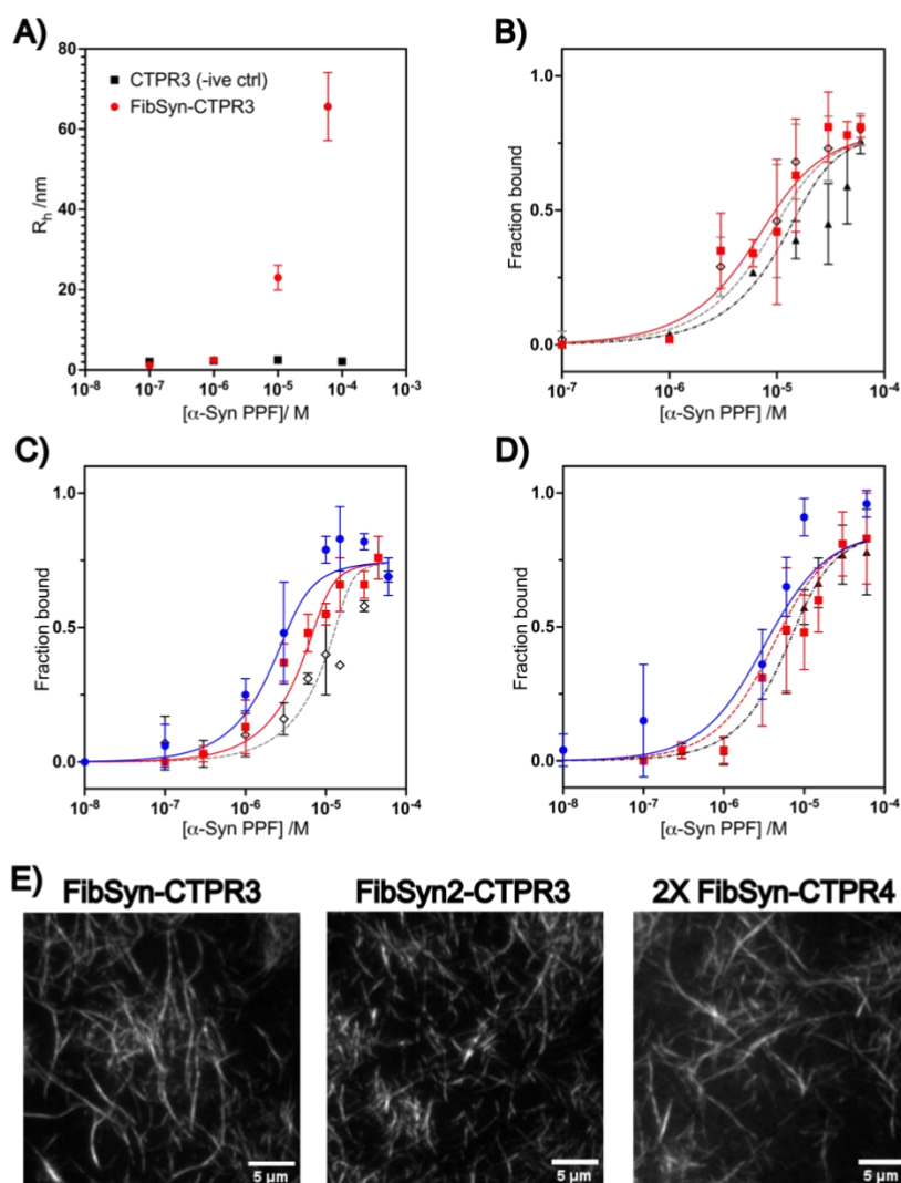
Figure 4: Microfluidic diffusional sizing (MDS) assay to determine binding affinity between fluorescently labelled CTPR variants and \alpha -synuclein preformed fibrils (PFFs). A) Initial hydrodynamic radius measurements to compare CTPR3 (negative control) and FibSyn-CTPR3 interactions with increasing \alpha -synuclein PPF concentrations. The hydrodynamic radius for FibSyn-CTPR3 significantly
