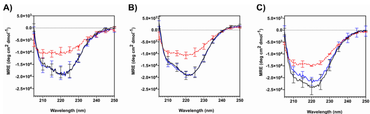
Figure 2: CD analysis of CTPR variant secondary structure. Far-UV CD spectra of A) FibSyn-CTPR3, B) FibSyn2-CTPR3 and C) 2XFibSyn-CTPR4 at 20°C (black), 90°C (red) and returning to 20°C (blue). Protein concentration was 5 \mu\text{M} in 50 mM sodium phosphate pH 7.5, 150 mM NaCl. Error bars are standard deviation calculated from three independent experiments.
