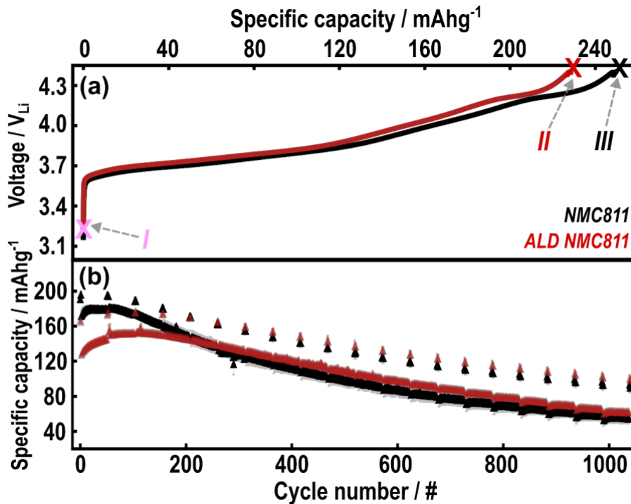
Figure 3: (a) Voltage profile of the first charge ( C/20 rate assuming 200 \text{ mAhg}^{-1} practical capacity) for NMC811 (black) and ALD NMC811 (red) where crosses indicate sample states analysed with post-mortem NMR: pink cross (I) indicates the ALD NMC811 soaked in 1 \text{ M LiPF}_6 in EC/EMC, the red cross (II) indicates the ALD NMC811 charged to 4.4 \text{ V}_{\text{Li}} (rinsed with DMC), and the black cross (III) is the NMC811 charged to 4.4 \text{ V}_{\text{Li}} (rinsed with DMC). Discharge capacities over long-term cycling in sets of 49x ageing cycles at C/2 and 2x diagnostic cycles at C/20 are presented in (b) for the NMC811 and ALD NMC811.
