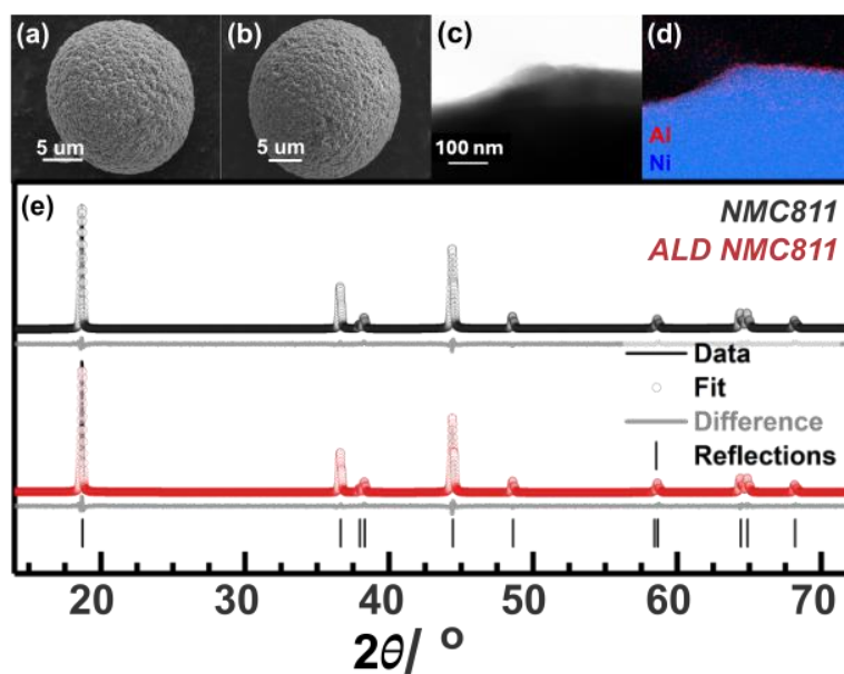
Figure 1: SEM images of the as-synthesised (a) NMC811 and (b) the ALD NMC811 secondary particles (c) Bright field image of an ALD NMC811 particle with (d) a corresponding EDX map of Ni (blue) and Al (red). The X-ray ( \lambda = 1.5406 \text{ \AA} ) diffraction patterns (e) of the NMC811 (black) and ALD NMC811 (red) are compared, showing the experimental data (solid line), the Rietveld refinement (open circles), the difference between the data and fit (grey line) and the position of the expected reflections of the R\bar{3}m space group (vertical ticks).
