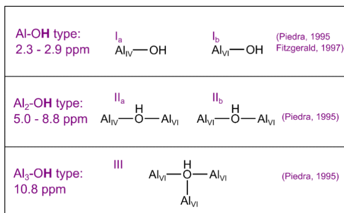
Scheme 1: The five different types of hydroxylated Al environments on the surface of \gamma -Al 2 O 3 proposed by Peri. 74 The references mentioned have assigned chemical shifts for these environments based on experimental data: Piedra et al. 75 and Fitzgerald et al. 76 Al IV denotes Al with tetrahedral coordination whilst Al VI denotes octahedral coordination.
