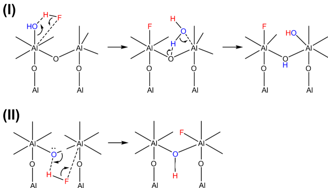
Scheme 3: Two different scenarios in which HF scavenging could occur on the hydrated Al 2 O 3 coating: (I) involves reaction with a terminal OH group that results in fluorination of an Al group with no change in coordination number. Water is released, which can react with a lower coordinate Al site nearby, resulting in an increase in the coordination number of this Al site and (II) a reaction involving fluorination of an undercoordinated site to increase its coordination number. The mechanisms presented here are based on basicity arguments, Al-F bonds strengths and the DFT predictions from Tebbe and co-workers. 47 . Hydroxyl groups on the Al groups not involved in the reaction are omitted.
