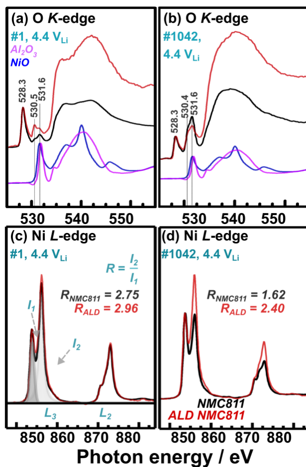
Figure 7: The O K-edge (a) and (c) Ni L-edge X-ray absorption spectroscopy of the NMC811 (black) and ALD NMC811 (red) electrodes charged to 4.4 V Li on the first cycle are presented with spectra from reference samples of \gamma -Al 2 O 3 (magenta) and NiO (blue). O K-edge and Ni L-edge spectra of the materials in the electrochemically aged state (after cycle 1042) and charged up to 4.4 V Li are presented in (b) and (d) respectively. Ratios of the L 3 high energy (I 2 , 855.8 eV) : low energy (I 1 , 853.7 eV) integrated areas are expressed with R for the Ni-Ledge.
