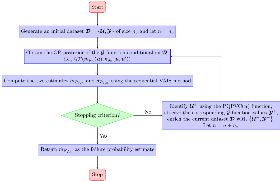
Fig. 2. Flowchart of the proposed QBALC method.
