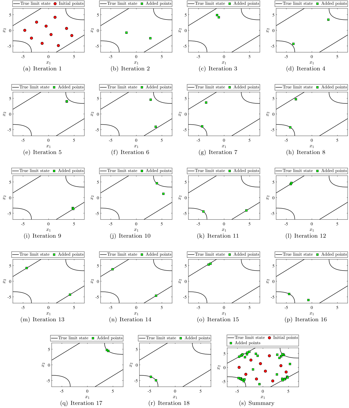
Fig. 3. Illustration of the proposed QBALC method ( n_a = 2 and \sqrt{\bar{\rho}} = 0.50 ) for Example 1.
