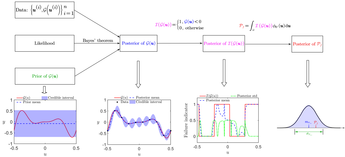
Fig. 1. Schematic diagram of the BFPI framework in standard normal space.
