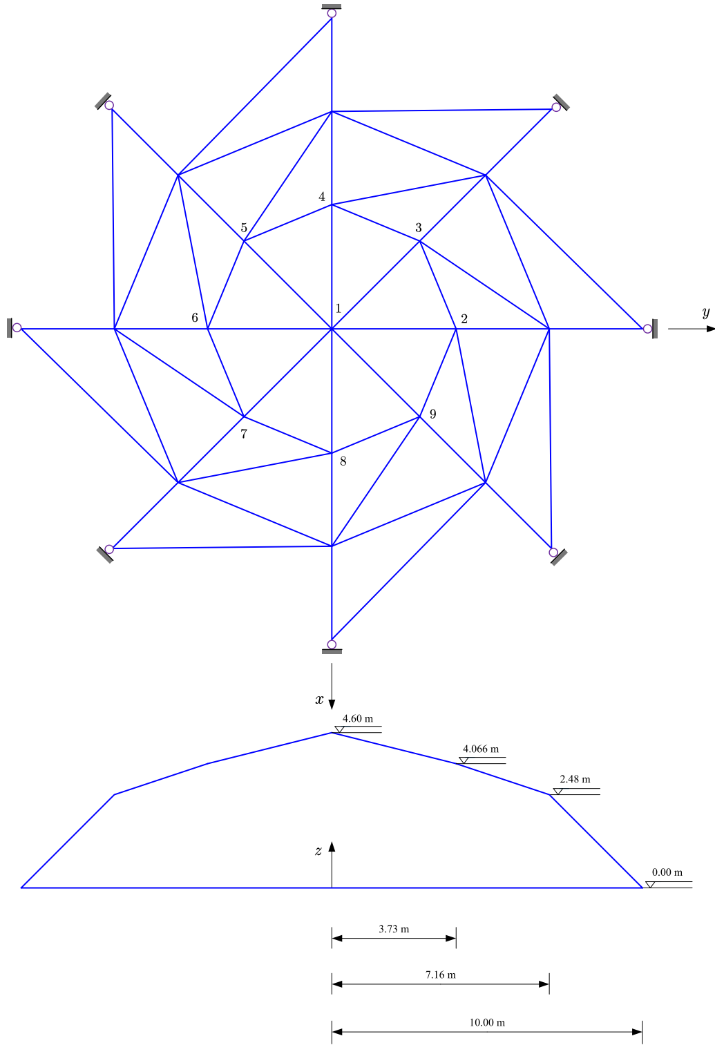
Fig. 6. Schematic of a 56-bar space truss structure.
