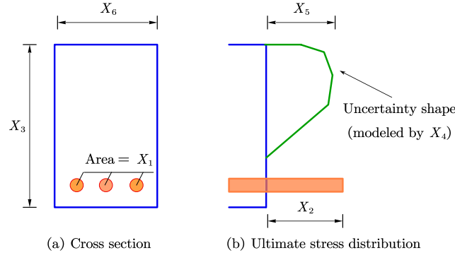
Fig. 5. Ultimate stress state of the reinforced concrete section.
