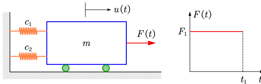
Fig. 4. A nonlinear single-degree-of-freedom oscillator under a rectangular pulse load.
