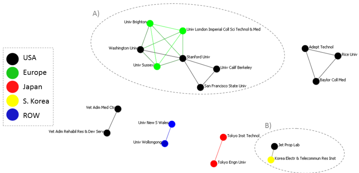
Figure 2: Collaboration networks (1983 – 1994)
