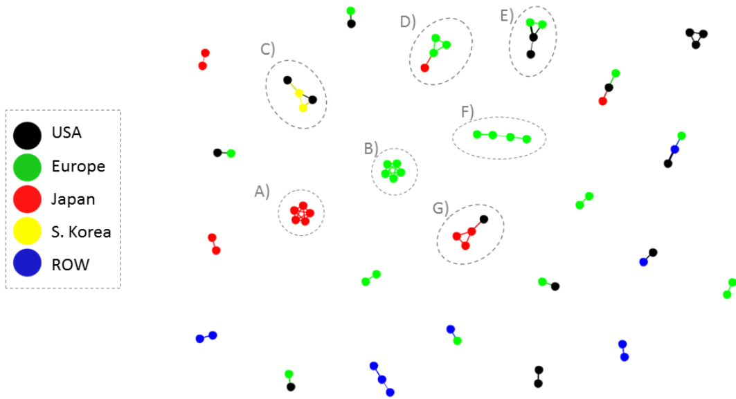
Figure 3: Collaboration networks (1995 – 1999)
