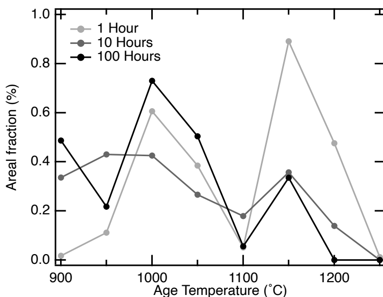
Figure S1: Total areal fractions of precipitates as a function of heat treatment temperature calculated from the data presented in Figure 7.
