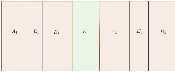
Fig. 3 Claim in the proof of Theorem 3.17
