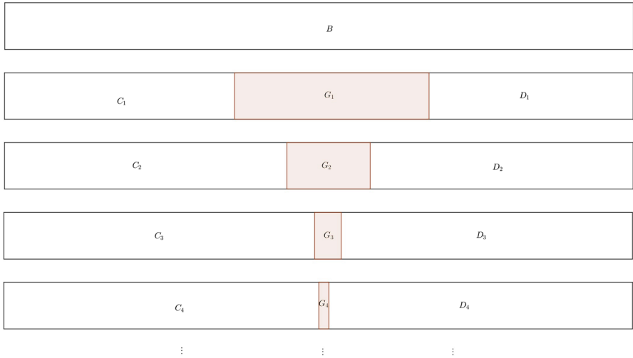
Fig. 1 Savage’s error reducing partitions
