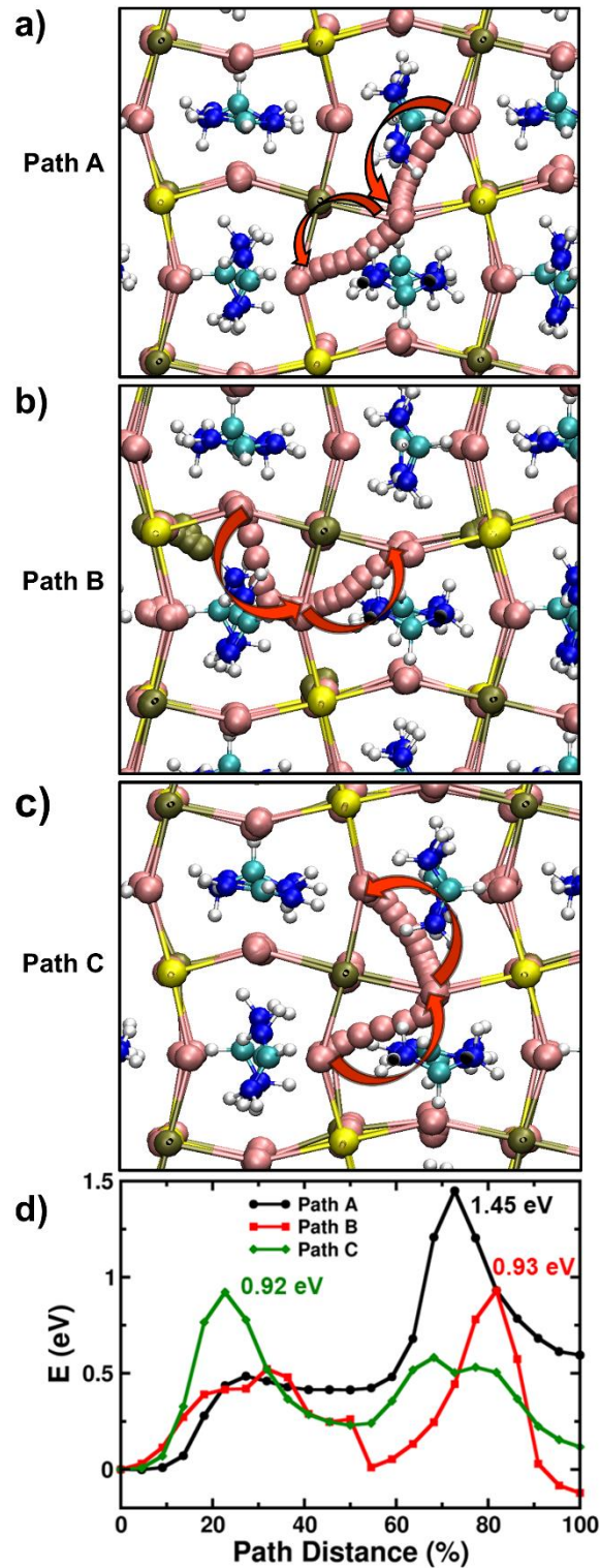
Figure 4: Ion migration pathways through atomistic ab initio simulations. a-c) Inequivalent iodide migration paths (A, B and C) in FAPb 0.5 Sn 0.5 I 3 involving the SnI 2 Schottky-type defect comprised of a Sn vacancy and two I vacancies. Here, brown, olive, pink, turquoise, blue and white spheres represent lead, tin, iodine, carbon, nitrogen and hydrogen atoms respectively. The red arrows point to the direction of iodide migration in the lattice. d) Energy profiles for iodide ion migration via paths A, B and C in FAPb 0.5 Sn 0.5 I 3 .
