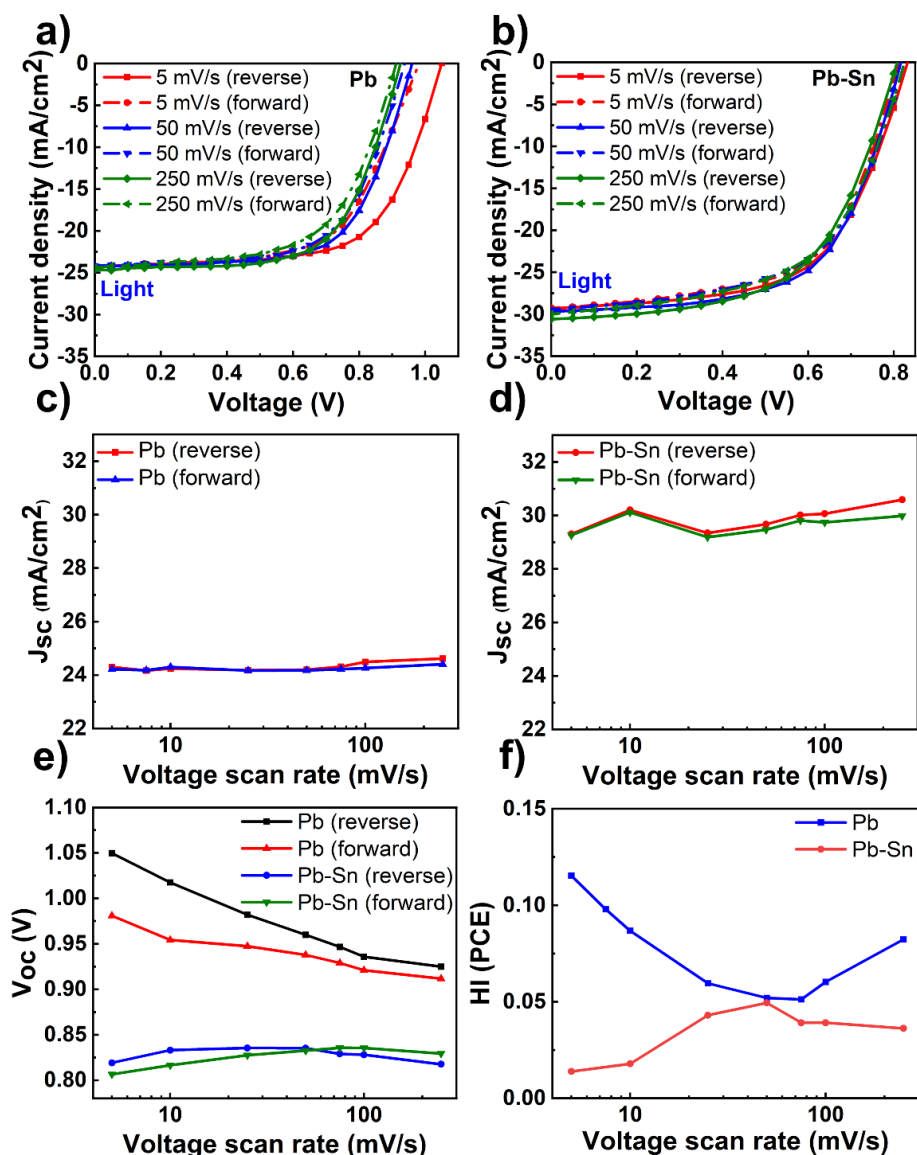
Figure 2: Scan-rate dependent J-V measurements. Light J-V scans of a) Pb and b) Pb-Sn perovskite solar cells at three scan rates: 5 mV/s, 50 mV/s and 250 mV/s. c) J sc of Pb perovskite solar cells as a function of scan rates in the reverse and forward scans. d) J sc of Pb-Sn perovskite solar cells as a function of scan rates in the reverse and forward scan. e) Open circuit voltage of Pb and Pb-Sn perovskite solar cells as a function of scan rates in the reverse and forward scans. f) Hysteresis index (HI) in PCE of Pb and Pb-Sn perovskite solar cells as a function of scan rates. Note that optimized 2PACz and PEDOT:PSS were used as HTLs respectively for Pb and Pb-Sn perovskite solar cells.
