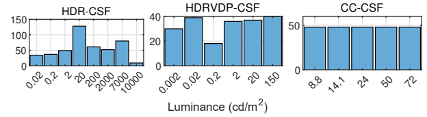
Figure 4. Number of data points across luminance levels in each dataset
