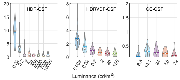
Figure 8. \Delta E_{2000}^G error predictions for 1 JND colour difference data points from the three dataset. Same notation as Figure 5
