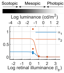
Figure 1. Values of rod contribution parameters as functions of retinal illuminance in trolands. \alpha_1 is the weight of rod contribution to L and M cones. \alpha_2 is the weight of rod contribution to S cones. The solid lines are fitted logistic functions. Data points are from Fig. 3 in Cao et al. [12] for two observers. We used the mean of the values to fit the logistic function. We have also shown the equivalent luminance in \text{cd/m}^2 and the approximate range for scotopic, mesopic and photopic regions.
