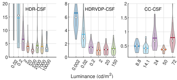
Figure 6. \Delta E_{2000}^{LMS} error predictions for 1 JND colour difference data points from the three dataset. Same notation as Figure 5
