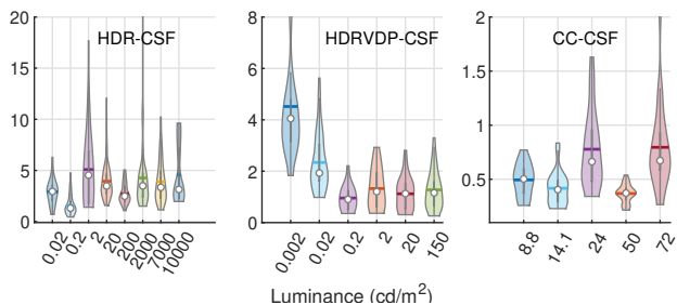
Figure 7. \Delta E_{2000}^{L'M'S'} error predictions for 1 JND colour difference data points from the three dataset. Same notation as Figure 5
