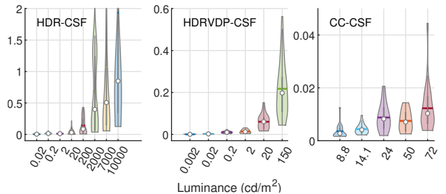
Figure 5. \Delta E_{LMSR} error predictions for 1 JND colour difference data points from the three dataset. The violin shapes show the smoothed kernel density at each error value. The white circles are the median and the horizontal lines are the mean values. The vertical grey lines show the interquartile range of the errors. The same notation is used in the subsequent violin plots. A well-performing colour difference metric should result in similar error values across the luminance levels (the mean and median values would approximately lie on a straight line).
