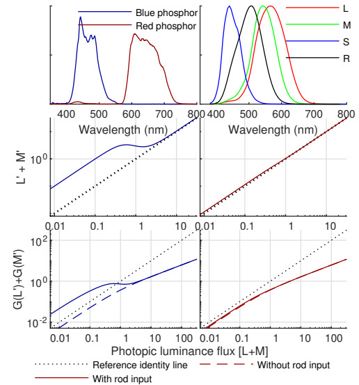
Figure 2. Demonstration of Purkinje shift using the modified photoreceptor response model. The blue and red coloured lines correspond to responses for blue and red display primary respectively. Top row (left): Emission spectra of blue and red display primaries. Top row (right): Spectral sensitivities of cones and rods. Middle row: Luminance from modified long and medium cone response L' + M' from Eq. (1). Bottom row: Luminance from regulated long and medium cone response G(L') + G(M') from Eq. (3).
