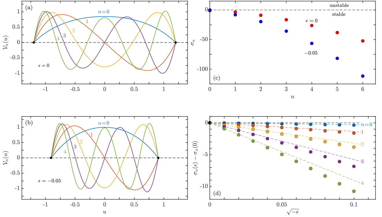
FIG. 9. Linear stability problem for mean curvature flow of subcritical and critical catenoids. First five eigenfunctions V_n(u) of the linear operator (33) for (a) the critical catenoid ( \epsilon = 0 ), and (b) a weakly subcritical catenoid ( \epsilon = -0.05 ). (c) Growth rates \sigma_n for the cases in (a) and (b) for the first 7 modes. When \epsilon = 0 , mode 0 is neutral and all others are stable, while for \epsilon < 0 all are stable. (d) Shifts in growth rates versus \sqrt{-\epsilon} (circles) compared to leading-order corrections (dashed) from (42).
