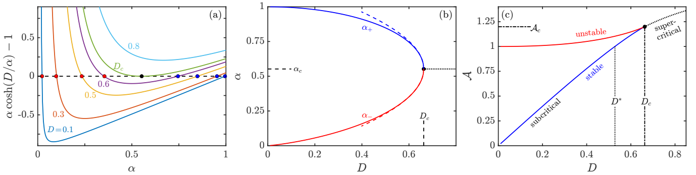
FIG. 8. Catenoid stability. (a) Solution of transcendental equation at various values of scaled loop separation D . (b) Two branches (red, blue) of solutions for \alpha as a function of D for subcritical catenoids, terminating at D_c = 0.6627\dots with \alpha_c = 0.5524\dots , and continuation (dotted) with \alpha = \alpha_c for supercritical ones. (c) Scaled area \mathcal{A} of catenoids along the two subcritical branches, terminating at \mathcal{A}_c = 1.199\dots at the critical separation D_c . The dotted line beyond D_c indicates the area of the family of stretched catenoids (20) given in (21).
