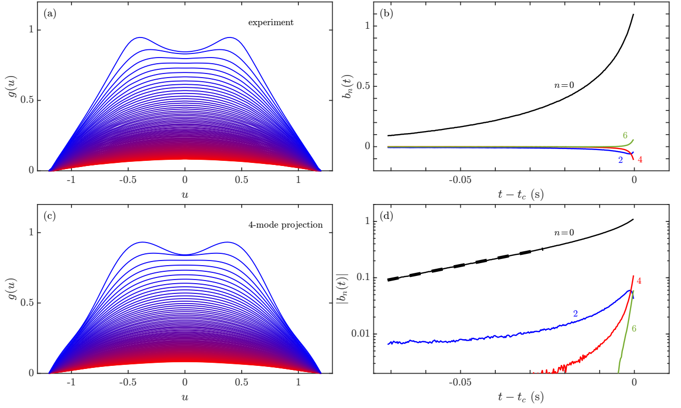
FIG. 12. Projection of experimental collapse dynamics onto modes. (a) The perturbation function g(u) as defined in (27), corresponding to the deviation of the interface shape from the critical catenoid, as a function of u = z/a , color-coded by time as in Fig. 6 from red (early) to blue (later). (b) Projection amplitudes for the first 4 even modes as a function of time relative to critical time t_c . (c) Reconstruction of the interface evolution using the mode amplitudes in (b). (d) As in (b), but a semilog plot of the absolute values of the mode amplitudes. Heavy dashed line is linear fit to extract mode growth rate.
