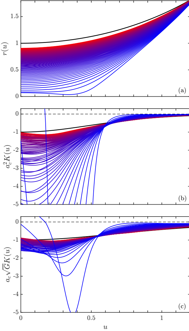
FIG. 6. Shape evolution and Gaussian curvature. (a) Shapes of collapsing catenoid in upper right quadrant, with film viscosity 4.3 mPa, as a function of scaled coordinate u = z/a_c from early time until development of cone. Spacing between contours is 0.75 ms, with colors transitioning from red (early) to blue (later). (b) Nondimensionalized Gaussian curvature and (c) product of K and surface metric for shapes in (a). Black curves in (a)-(c) are quantities for equilibrium catenoid.
