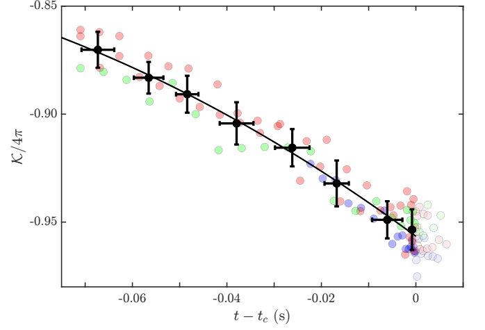
FIG. 7. Time evolution of the total curvature of collapsing catenoids. Data shown follows color scheme in Figs. 3 and 4 with reduced intensity. Solid black circles with error bars (standard deviations) are binned averages of the data sets. Black curve is a low-order polynomial fit to the data.
