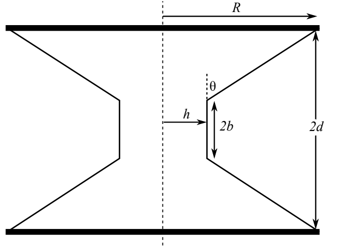
FIG. 13. Martini-glass approximation to the soap film surface.
