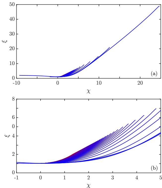
FIG. 16. Test of similarity solution. Data used in Figs. 6 and 12 are plotted in similarity variables (89) with same color scheme as before. (b) is enlargement of central region of (a).
