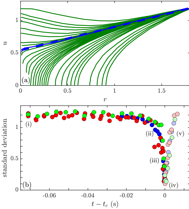
FIG. 4. Determination of the critical time for appearance of Martini glass configuration. (a) Film profiles (green) in the top-right quadrant. Profile corresponding to the Martini-glass configuration is blue and its linear interpolation (dashed blue) defines the angle \theta^* . (b) Standard deviation of the angle obtained by linear interpolation vs. time relative to critical time t_c . Inset displays values centered around the local minimum. Same color scheme and labelling convention as in Fig. 3.
