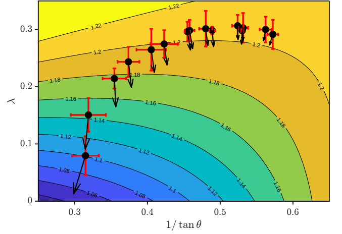
FIG. 14. Mapping experimental data onto the sequence. Contour plot of the energy function S in the parameter space of cone angle \theta and scaled radius \lambda . Arrows on experimental data points indicate -\nabla S .
