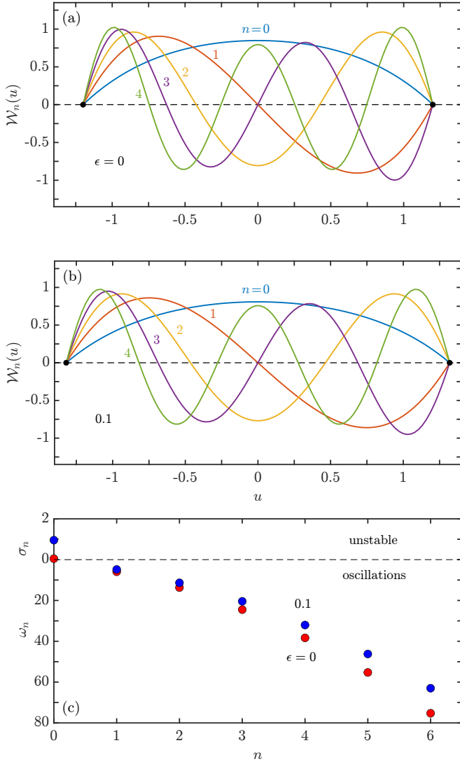
FIG. 11. The linear stability problem for Euler flow for critical and supercritical catenoids. (a,b) First five eigenfunctions \mathcal{W}_n(u) of the linear operator in (61) for a the critical catenoid ( \epsilon = 0 ) and a weakly supercritical one ( \epsilon = 0.1 ). (c) Growth rates \sigma_n and oscillation frequencies \omega_n for the first seven modes for the cases in (a) and (b). Note the frequency scale ( \omega_n ) increase downward, while the growth rate scale ( \sigma_n ) increased upward and is magnified by a factor of ten.
