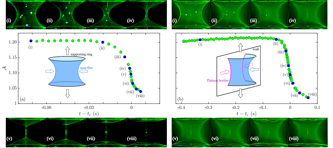
FIG. 2. Collapse dynamics of three dimensional catenoid compared to that of a hemi-catenoid in contact with a glass plate. (a) Time evolution of the scaled area \mathcal{A} (where \mathcal{A} = (\text{film area})/2\pi R^2 and R is the hoop radius) as the film evolves from the original catenoid to two discs. Points labelled (i-viii) correspond to characteristic stages in the evolution shown in the respective images. (b) As in (a), for the hemi-catenoid collapse. Note the much longer time scale for collapse compared to (a).
