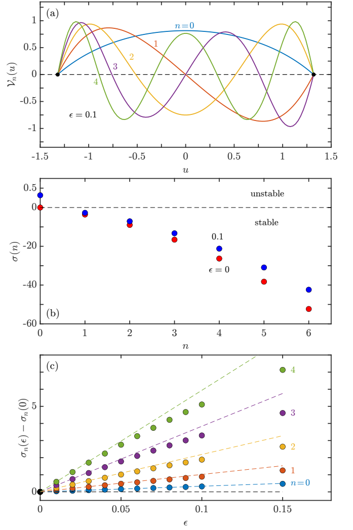
FIG. 10. Linear stability problem for MCF of supercritical catenoids. (a) First five eigenfunctions of the operator (50b) for a weakly supercritical case ( \epsilon = 0.1 ). (b) Growth rates \sigma_n for the first seven modes. When \epsilon = 0 , mode 0 is neutral and all others are stable; for \epsilon > 0 mode 0 becomes unstable while others remain stable. Note scale shift for positive \sigma axis. (d) Shifts in growth rates (solid symbols) compared to leading-order linear corrections arising from (53) (dashed lines).
