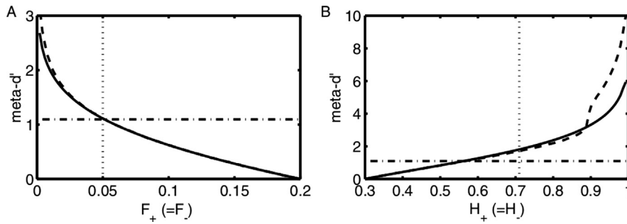
Fig. 1. Simulated data demonstrating the behaviour of meta- d' under systematic variation of Type II false alarm and hit rates. For both graphs, meta d' balance (an analytical version of meta d' ) is a solid line, and meta d' SSE is the dashed line. Dashed-dotted lines show d' . The vertical dashed line in this simulation is the boundary where the measure becomes unreliable (clearly non-linear). (A) Shows meta- d' against type II false alarm rate. (B) Shows meta- d' against type II hit rate. Note that, particularly for meta d' SSE, for high type II hit rates, meta d' becomes unreliable. For parameter and model details, see Fig. 5 from Barrett et al. (2013). Reproduced with permission.
