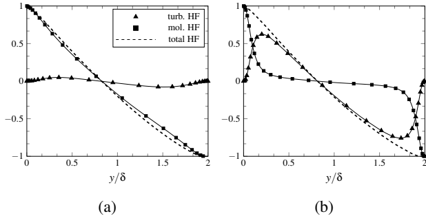
Fig. 5: Profiles of molecular (Pr^{-1}d\bar{\Theta}/dr)^+ , turbulent (\overline{v'\Theta'})^+ and total ((Pr^{-1}d\bar{\Theta}/dr) - \overline{v'\Theta'})^+ wall-normal heat flux; a) Pr = 0.026 b) Pr = 0.71
