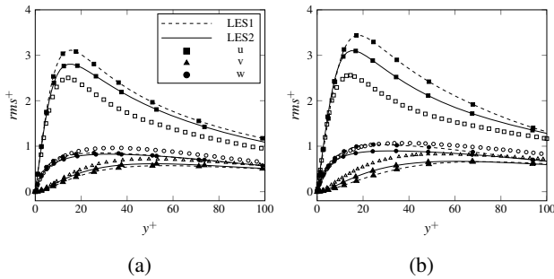
Fig. 4: Root mean square profiles (rms) of velocity fluctuations; a) inner b) outer; open symbols refer to DNS of Ref. [15]
