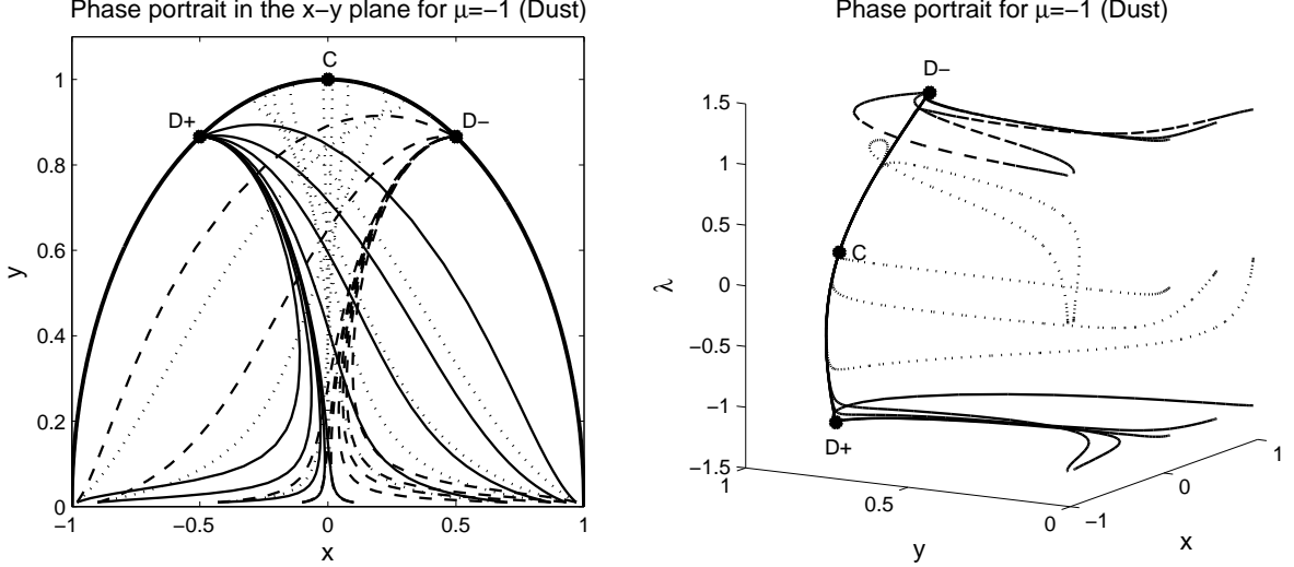
FIG. 4: Phase portrait in the x - y plane and in the E^3 space for the potential V(\phi) = V_0 \cosh^q(p\phi) with variables (p, q, w_m) = (-\frac{\sqrt{6}}{4}, 2, 0) , which corresponds to the integrable case for \mu = -1 . The point C is the unique stable point. The points D_{(\pm)} act as attractors in the plane (x - y) for \lambda = \pm \frac{\sqrt{6}}{2} . From the right-hand plot we observe that the solutions reach a boundary where \Omega_{m0} = 0 , w_\phi > -1 and from there they move to the de Sitter point C . The solid lines are for initial condition \lambda = pq , the dashed lines for \lambda = -pq , and the dotted lines for \lambda = 0 .
