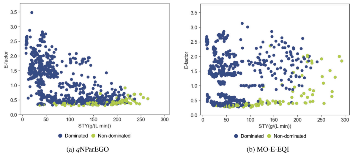
Fig. 10. Results of 20 repeated runs for qNParEGO and MO-E-EQI with Loglinear-2 noise structure. (a). Results of qNParEGO; (b). Results of MO-E-EQI. For both figures, the optimization started with 20 initial points and optimized for another 20 steps; the blue points are the dominated solutions from all 20 repeated runs and the green points are 20 Pareto front solutions all plotted at once.
