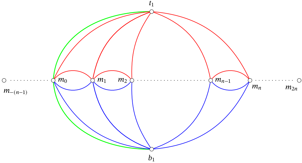
Fig. 1. Initial infection G_0 showing only the first top and bottom vertices, t_1 and b_1 . Each red or blue triangle represents an edge of G_0 , and together they form the first beachball hypergraph in our process. The green arc represents an edge containing the vertices it passes through. To form G_1 , the edge t_1b_1m_1 is added, as this completes a copy of K_4^{(3)} on \{t_1, m_0, m_1, b_1\} . It is clear to see that subsequently all edges of the form t_1b_1m_\ell for \ell increasing from 2 to n are added in turn. (For interpretation of the references to colour in this figure legend, the reader is referred to the web version of this article.)
