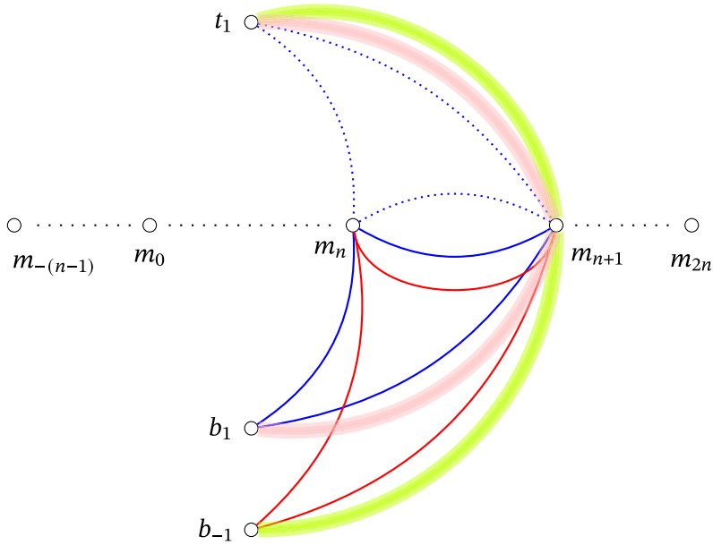
Fig. 2. Switching gadget to change from K_4^{(3)} copies containing b_1 to those containing b_{-1} . The edges b_1m_n m_{n+1} and b_{-1}m_n m_{n+1} are present in the initial infection G_0 . After the edge t_1 b_1 m_n is created by the percolation process, the copy of K_4^{(3)} induced by the vertices \{t_1, m_n, m_{n+1}, b_1\} is present, except for the missing edge t_1 m_n m_{n+1} shown in the dotted blue line. Thus this edge is added, followed by t_1 b_{-1} m_n . This triggers the process to run backwards and create all edges of form t_1 b_{-1} m_i , for i decreasing from i = n - 1 to i = 0 , in turn. (For interpretation of the references to colour in this figure legend, the reader is referred to the web version of this article.)
