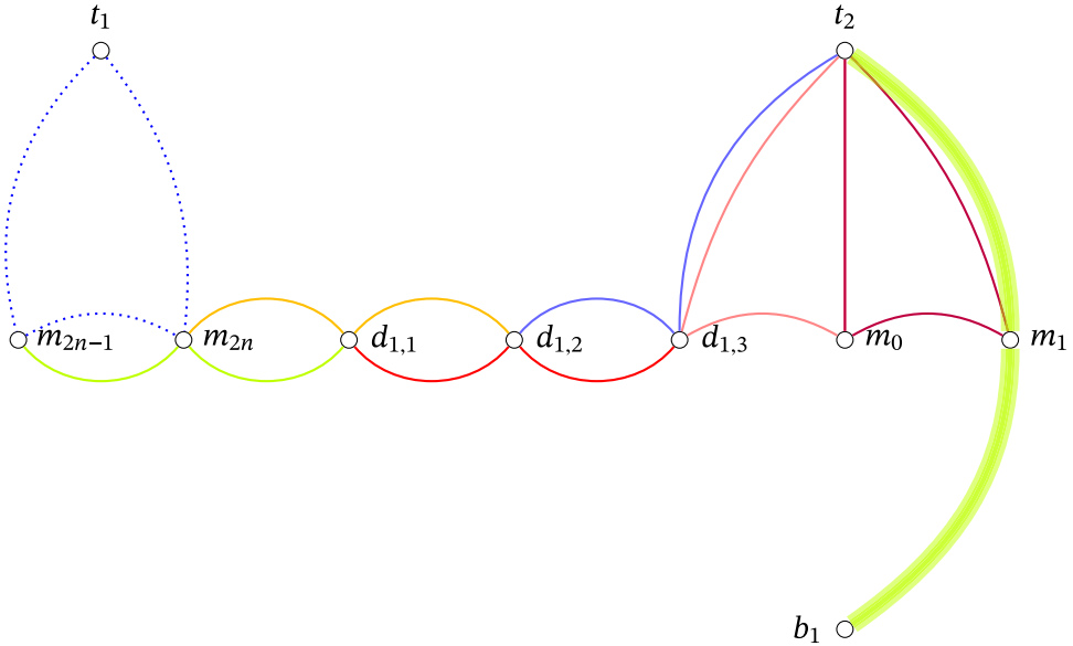
Fig. 3. Switching gadget for changing the top vertex t_1 to t_2 . Edges present in the initial infection G_0 are omitted for clarity. When the dotted blue edge t_1m_{2n-1}m_{2n} is infected, this causes the edges along the chain to become infected, ending in t_2m_0m_1 . This triggers the infection of t_2b_1m_1 , and in turn the process from the stage as shown in Fig. 1, with t_1 replaced with t_2 . (For interpretation of the references to colour in this figure legend, the reader is referred to the web version of this article.)
