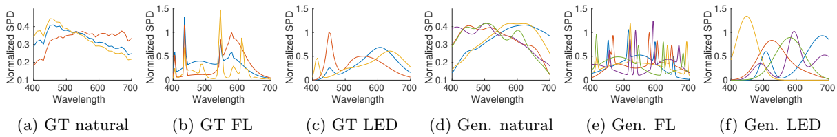
Figure 3: The comparison between CIE standard illuminants (left 3) and generated SPDs (right 3) for natural daylight, fluorescents and LEDs.
