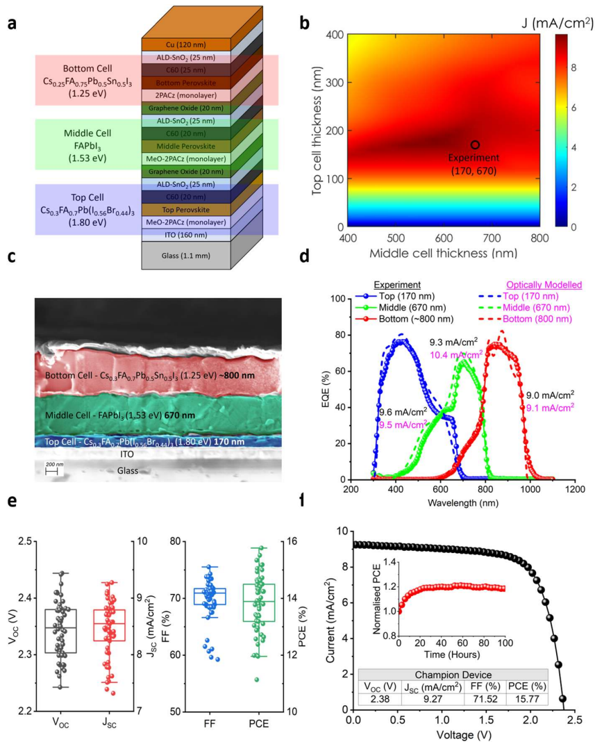
Fig. 2 | Demonstration of monolithic PPP triple-junction solar cells together with optical modelling
