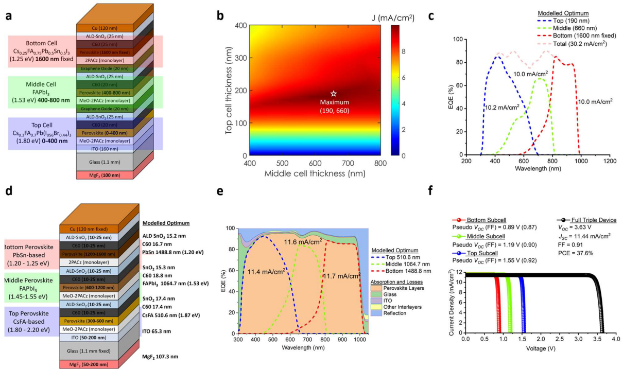
Fig. 3 | Further optimisation parameters for the demonstrated monolithic PPP triple-junction solar cell.
