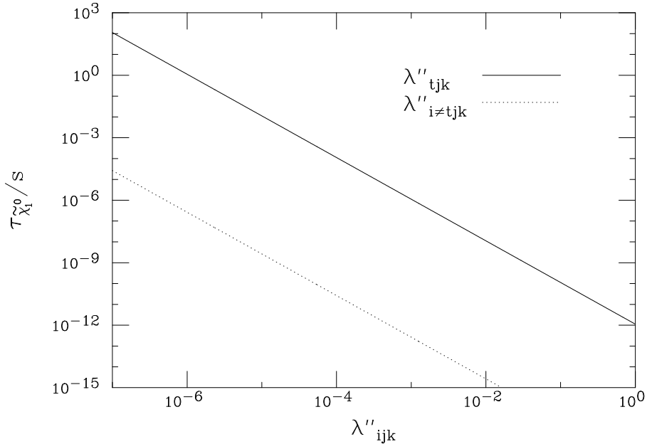
Figure 1: The lifetime of the \tilde{\chi}_1^0 at the mSUGRA point described in the text, with one of \lambda''_{ijk} non-zero. The solid line shows the lifetime for a dominant top quark coupling, which leads to the decay \tilde{\chi}_1^0 \rightarrow qq't^* \rightarrow qq'bW^* \rightarrow qq'bf' , where q and q' are quarks other than top and f and f' are Standard Model fermions. The dashed line shows the lifetime for couplings to quarks other than the top. The calculation approximates the final state particles as massless, so that the lines for \lambda''_{tjk} are the same for all j, k , as are those for \lambda''_{ijk} for all i \neq t, j, k .
