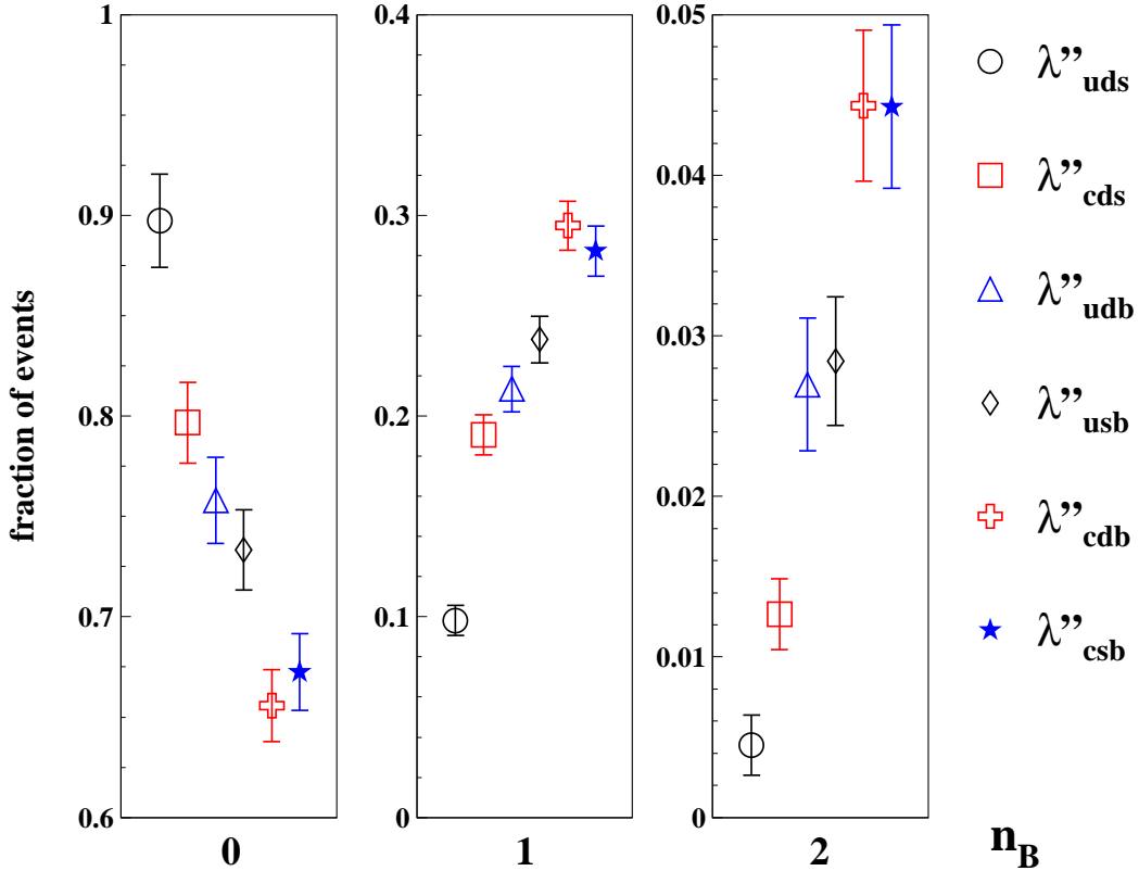
Figure 2: The fraction of signal events with 0, 1, and 2 vertex tags, for different types of RPV coupling \lambda'' . The statistical errors are those expected for an integrated luminosity of 30 \text{ fb}^{-1} . Points are horizontally displaced to allow them to be distinguished by eye.
