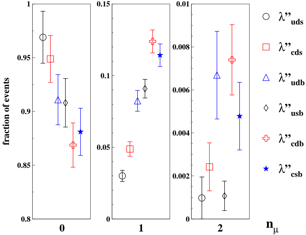
Figure 3: The fraction of signal events with 0, 1 and 2 muons that lie within \sqrt{\Delta\eta^2 - \Delta\phi^2} \leq 0.4 of the signal jets, for different types of RPV coupling, \lambda'' . The statistical errors are those expected for an integrated luminosity of 30 \text{ fb}^{-1} . Points are horizontally displaced to allow them to be distinguished by eye.
