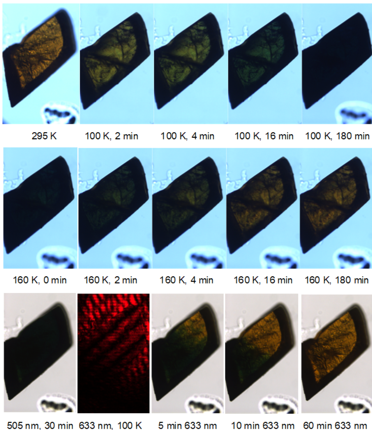
Figure 3 - Single-crystal optical microscopy images of the crystal of 1 (top) upon the application of t minutes of 505 nm light at 100 K; which is then (middle) warmed to 160 K and monitored as a function of time elapsed at 160 K; (bottom) upon the application of 30 min of 505 nm light while at 100 K, to which t min of 633 nm light is then applied.
