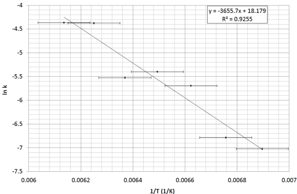
Figure 4 - Arrhenius plot of 1/T versus \ln k whose gradient ( E_a/R ) yields an activation energy, E_a = 30(1) kJ/mol.
