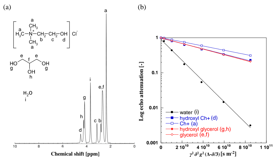
Figure 4. (a) ^1\text{H} NMR spectrum of aqueous Glyceline at 13 wt% water content at 20 °C . The NMR peak positions are (in ppm): a = 2.40; b = 2.81; c = 3.13; d = 4.50; e,f = 2.67; g = 4.17, h = 4.25, i = 3.68. All resonances are quoted relative to the ^1\text{H} resonance of tetramethylsilane (TMS). (b) PFG NMR log attenuation plots for the various species in aqueous Glyceline with a 13 wt% fraction of water. The letters in brackets in the legend refer to the peak assignment made on Figure 4a. Note the distinctive diffusion attenuation of water relative to the other species. Solid lines are fittings using Equation (1).
