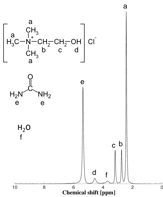
Figure 3. ^1\text{H} NMR spectrum of aqueous Reline at 1 wt% water content at 20 °C . The NMR peak positions are (in ppm): a = 2.43; b = 2.75; c = 3.18; d = 4.59; e = 5.38; f = 3.69. All resonances are quoted relative to the ^1\text{H} resonance of tetramethylsilane (TMS).
