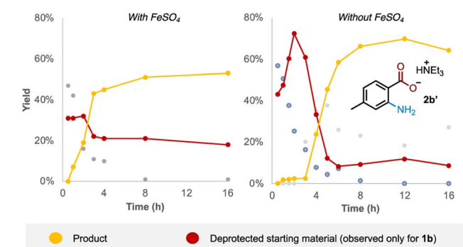
Fig. 3 Time course reaction profile for 1b with and without iron catalysis.
