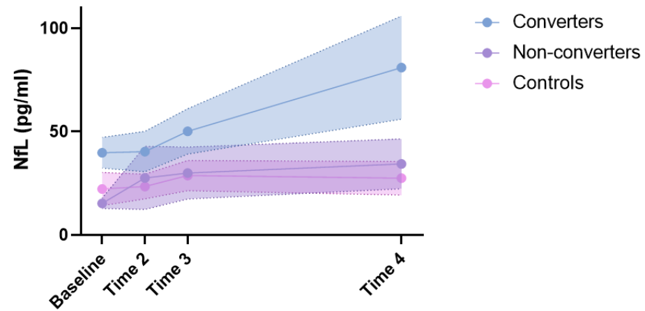
Bootstrapped Pooled Data (EMM, SEM) with Group ANOVA Results
