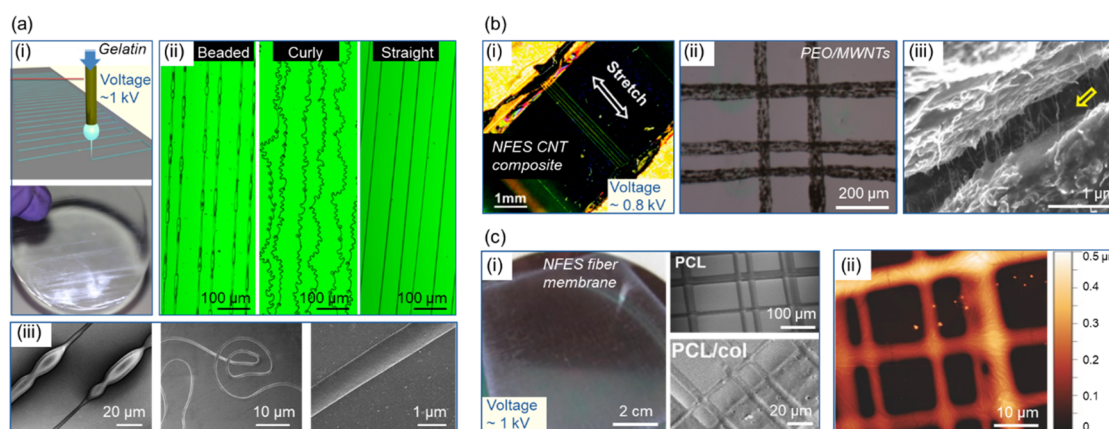
Figure 2. Near-field electrospinning of various biopolymers and carbon nanomaterials. (a) Versatile gelatin fibrous patterns created by the NFES approach: (i) schematic illustration of the NFES direct-writing approach, (ii) beaded, curly, and straight gelatin fiber patterns, and (iii) scanning electron micrographs showing typical regions of the fiber patterns. Reprinted with permission from ref 40. Copyright 2014 PLoS One. (b) Multiwalled carbon nanotubes (MWCNTs) composite polymer electrode printed by NFES: (i, ii) microscopic images showing the composite fibers in suspension and on a substrate, (iii) MWCNTs bridging an open crack along the fiber axis (the MWCNTs are shown by a yellow arrow). Reprinted with permission from ref 42. Copyright 2012 IOP Publishing. (c) PCL/collagen interconnected fiber membrane fabricated by NFES: (i) photo of the thin film, (ii) SEM micrographs of the interconnected PCL and PCL/collagen fibers, and (iii) atomic force microscope characterization of the PCL fiber network. Reprinted with permission from ref 34. Copyright 2018 John Wiley and Sons.
