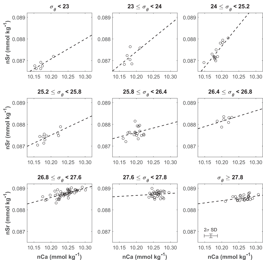
Fig. 5. nSr-nCa property-property plots along isopycnal surfaces in the North Pacific Ocean. Calcium data are from Steiner et al. (2021).
