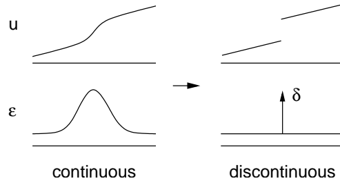
Figure 2: From continuous to discontinuous displacement/strain profiles as a consequence of strain localisation.
